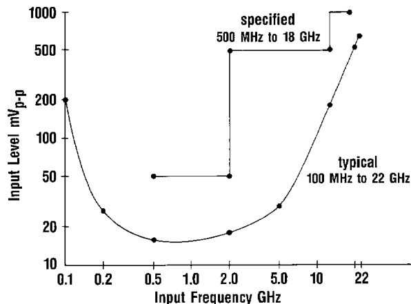
HP 54118A Sensitivity vs. Frequency While maintaining jitter specification
