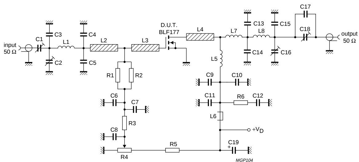
Fig.19 Test circuit for class-B operation.
