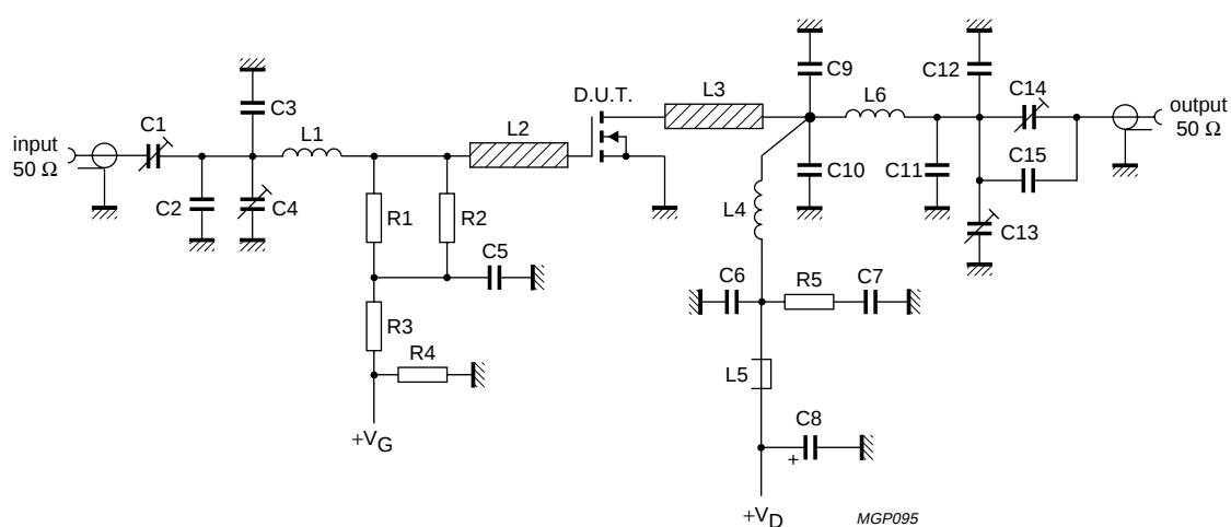
Fig.13 Test circuit for class-AB operation.
