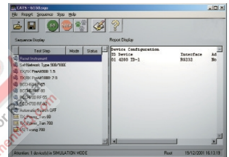
figure 4 CATS Software
