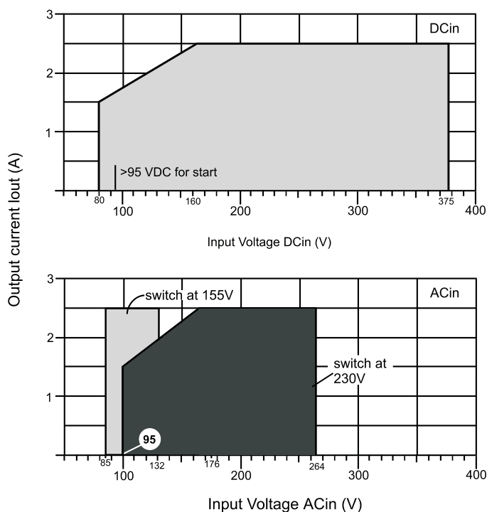
Output Current over Input Voltage (min.)
