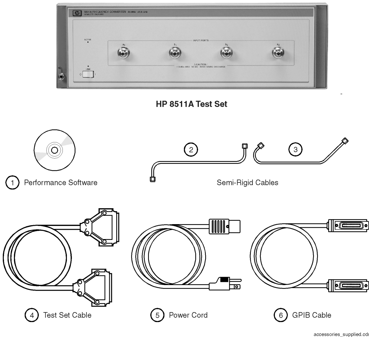
Figure 1-1 HP 8511A Test Set with Accessories Supplied
