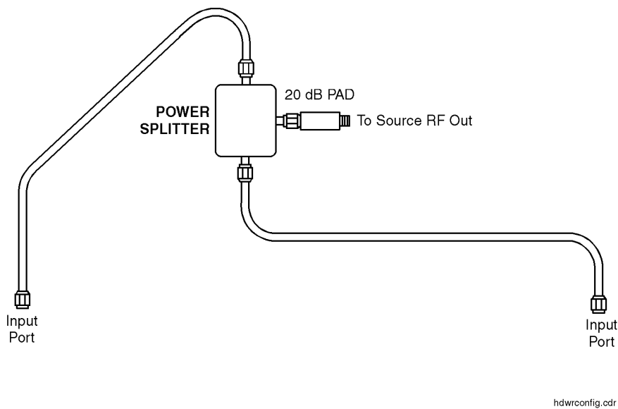
Figure 4-3 Hardware Configuration for Operator's Check
