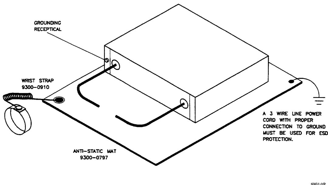
Figure 3-1 Static Safe Work Area
