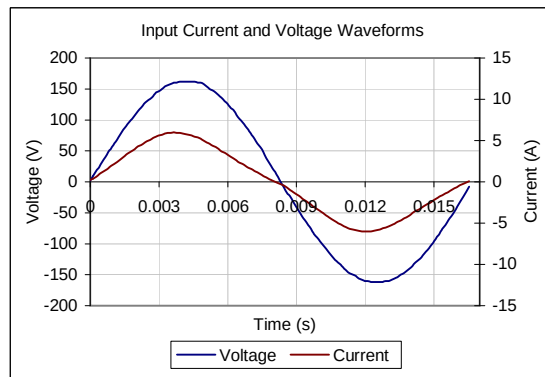
Input AC Current Waveform (ITHD = 16.1%, 50% Load)
