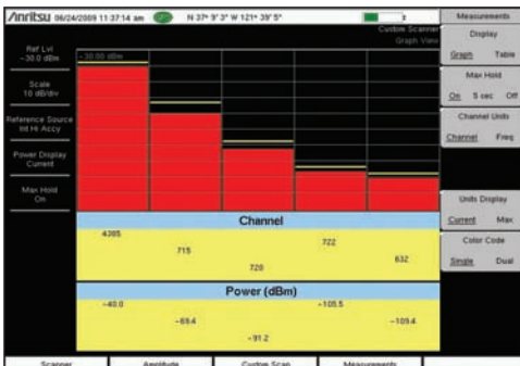
Channel Scanner
