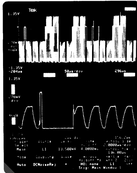
Two built-in time bases provide the functionality of delaying and delayed sweeps in analog scopes. The main time base defines the overall acquisition interval and the window time base allows high resolution acquisition of small portions of complex waveforms.
