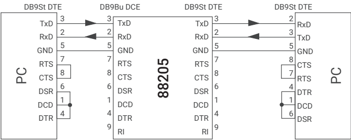
RS232 application with software handshake
