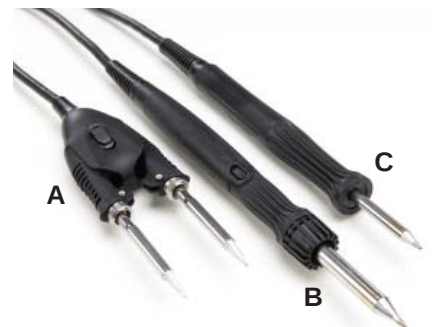
MFR-2200 Series Hand-pieces A. MFR-H4-TW Precision Tweezers B. MFR-H2-ST Soldering Tip C. MFR-H1-SC Soldering Cartridge
