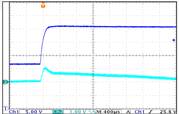
Figure 12: Output Voltage Response to Step-Change in Input Voltage, ( dV/dt = 250 V/ms). Load capacitance: 1 \mu F ceramic and 990 \mu F electrolytic capacitors. Ch 1: V_{in} (5 V/div); Ch 2: \Delta V_{out} (1 V/div). Timescale: 400 \mu s/div.
