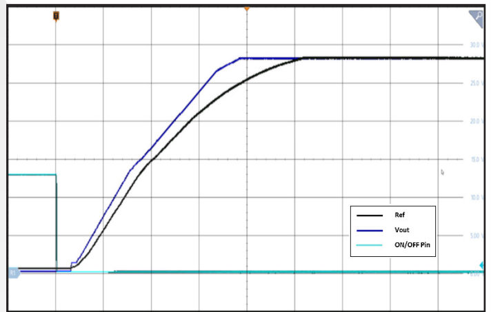
Figure 16: Hi-Cap Option Startup Waveform , input voltage pre-applied. Ch1: Vout, 470μF, no load (5V/div); Ref: Vout, 130mF, full resistive load (5V/div); Ch2: ON/OFF Pin (5V/div). Constant-current loads may significantly slow down the startup ramp when combined with large capacitances. Timescale: 100ms/div.
