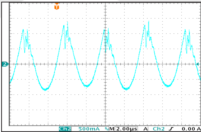
Figure 9: Input Terminal Current Ripple, i_c , at full rated output current and nominal input voltage with a 470 \mu F electrolytic capacitor (500 mA/div). Bandwidth: 20 MHz. Timescale: 2.00 \mu s/div. See Figure 13.
