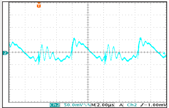
Figure 10: Output Voltage Ripple, V_{out} , at nominal input voltage and rated load current (50 mV/div). Load capacitance: 1 \mu F ceramic and 10 \mu F tantalum capacitors. Bandwidth: 20 MHz. Timescale: 2.00 \mu sec/div. See Figure 13.
