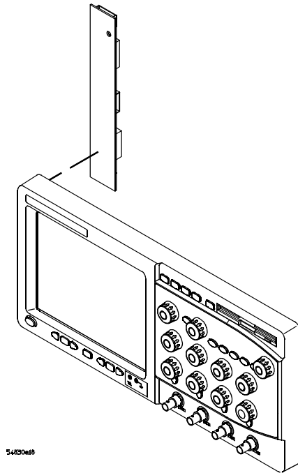
Backlight Inverter Board
