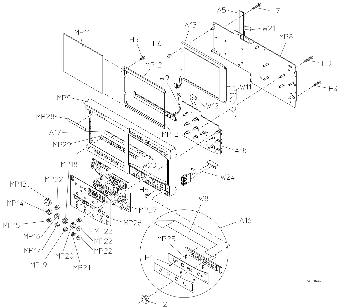
Front Frame and Front Panel
