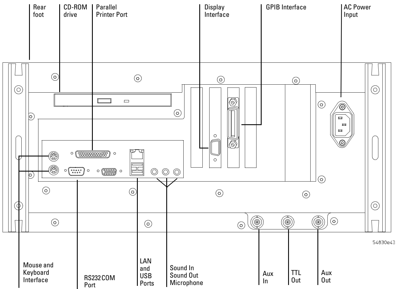
Rear Panel of 54830-series oscilloscope
