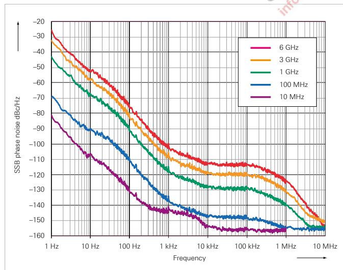
Measured SSB phase noise with internal OCXO (R&S®SMBV100A/B1 option)
