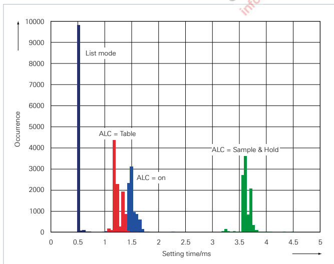
Histogram of measured level setting times in I/Q mode
