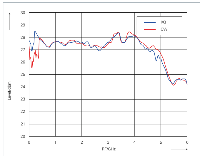
Measured maximum output power vs. frequency
