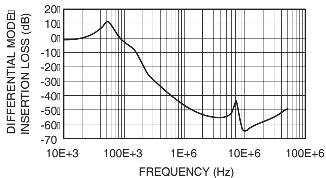
Figure 3. Typical Differential-Mode Insertion Loss in a 50 \Omega Circuit
