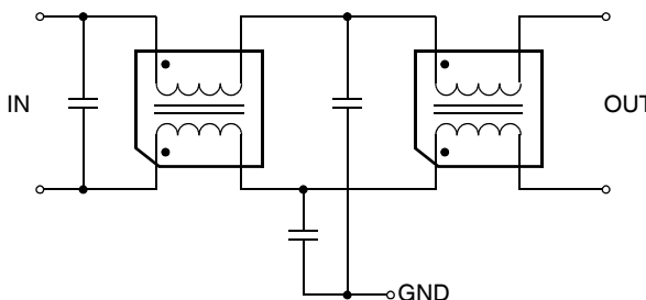
Figure 4. Internal Schematic
