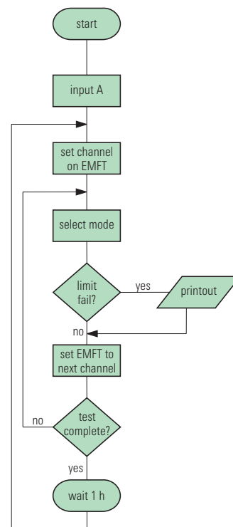
Example of AUTORUN routine
