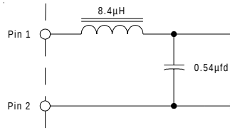
Figure IV. Input Filter Circuit
