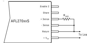
Figure V. Connection for V_{OUT} Adjustment
