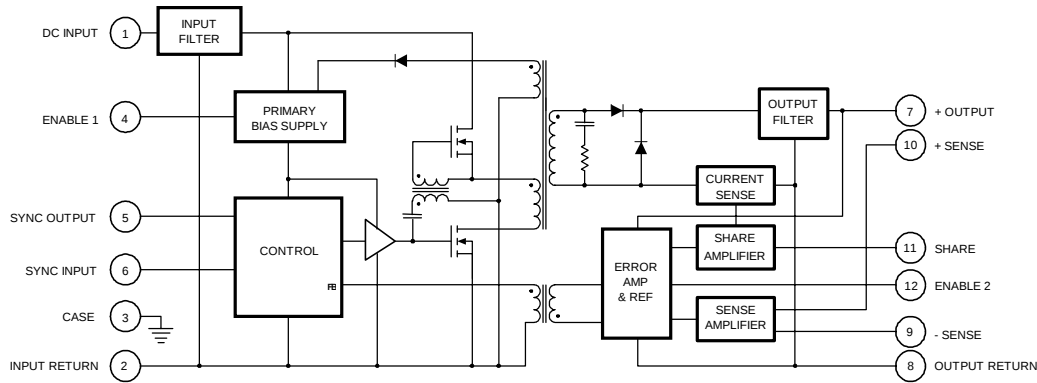
AFL270XXS Circuit Description Figure I. AFL Single Output Block Diagram
