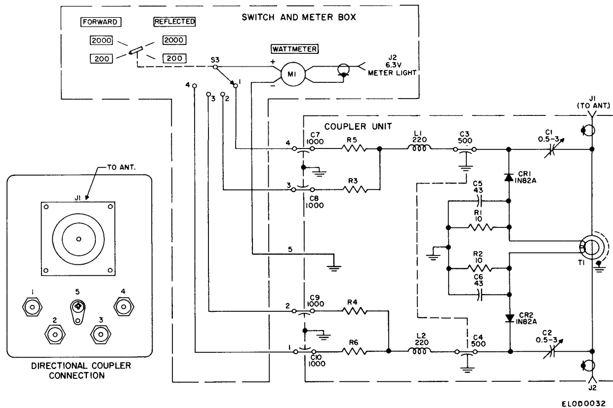
Figure 10-5. Wattmeter Interconnections.
