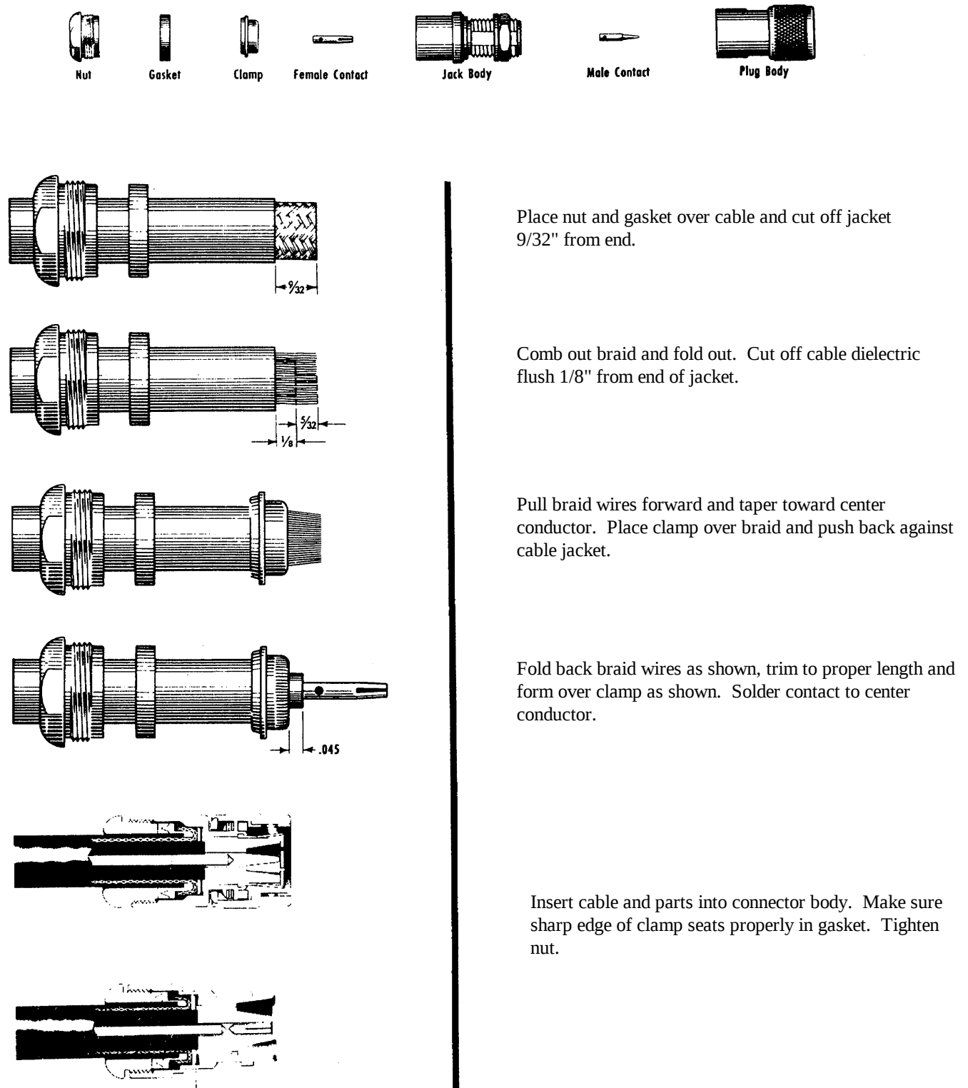
Figure 11-1. Connector assembly instructions.
