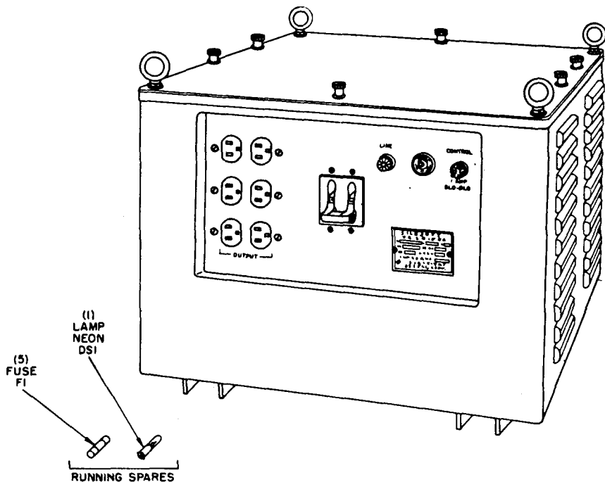
Figure 9-1. Regulator, Voltage CN-1214/G ,front panel view.
