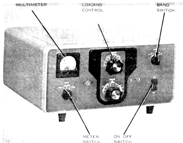
Figure 11-4. Collins 30L-1, operating controls.
