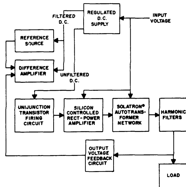
Figure 8-4. Regulator, Voltage , CN-1146/FRC -95, block diagram
