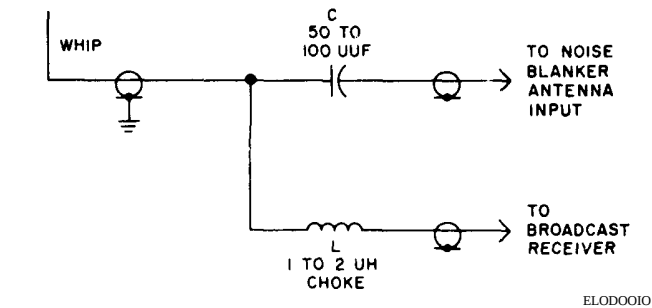
Figure 6-1. Suggested connections for using broadcast whip for both broadcast receiver and noise blanker.
