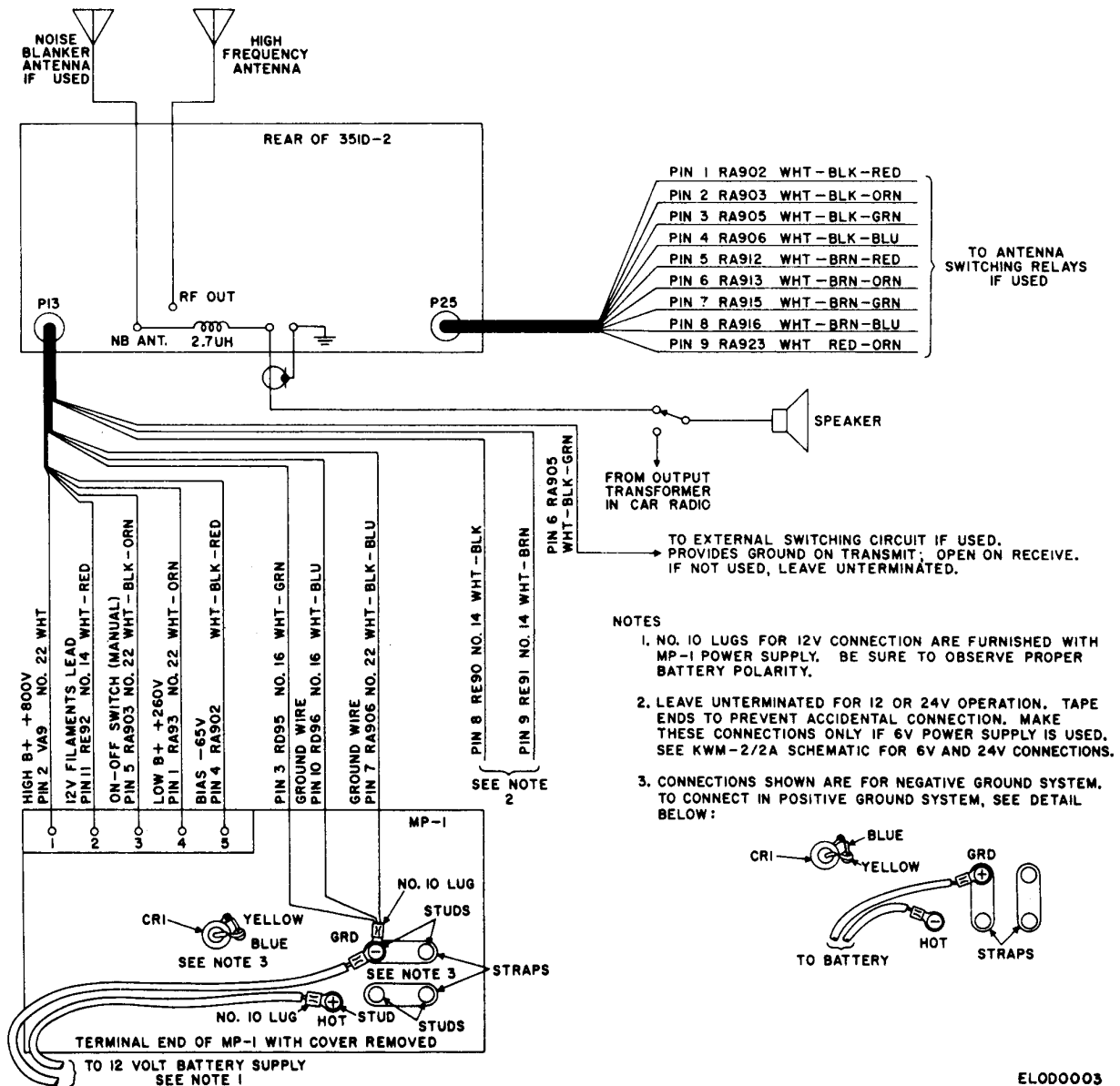
Figure 3-3. Mobile station interconnections.
