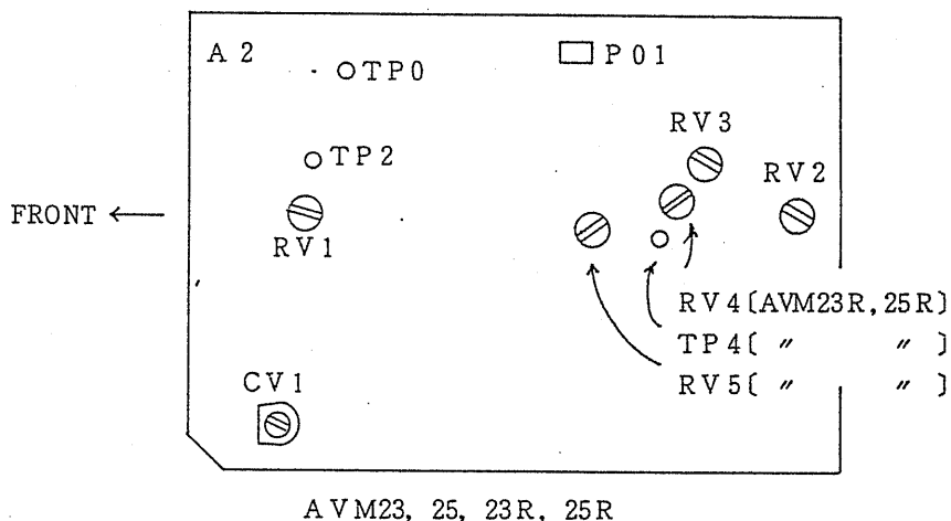
Figure 5 A2 (Dual-pointer models only)
