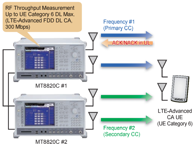
Sample MT8820C connection
