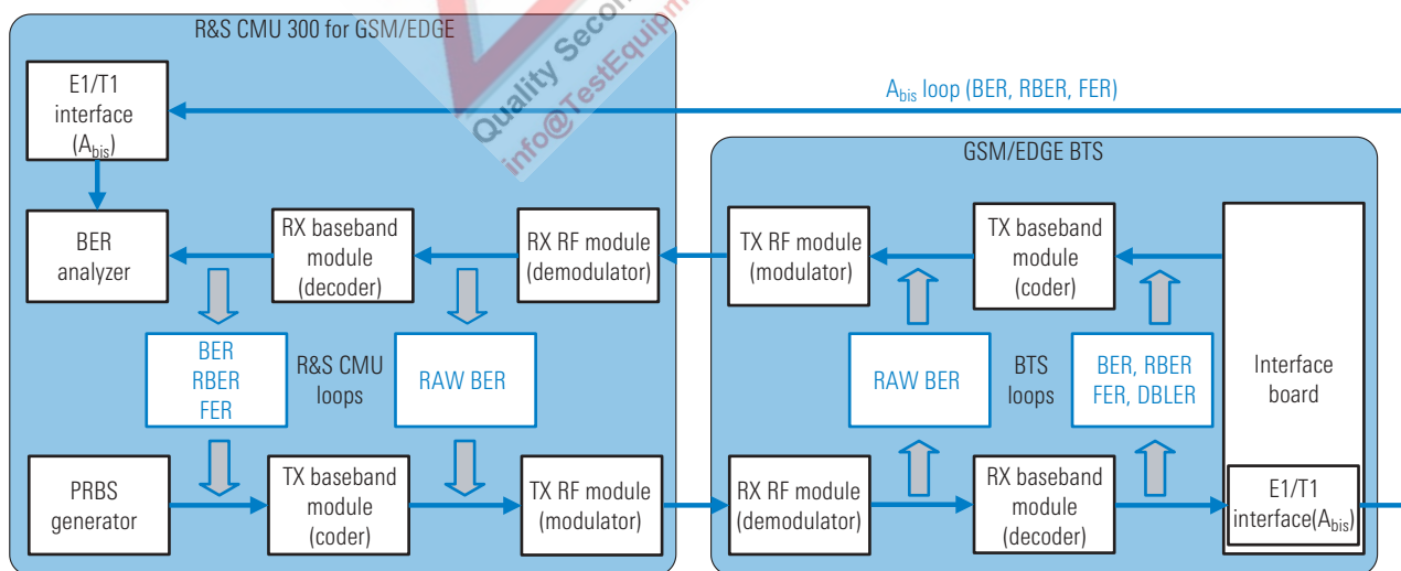
BER test environment
