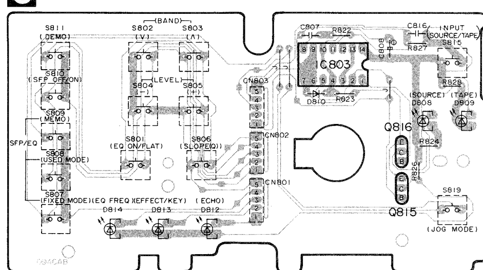
C OPERATION P.C.B. (REP1460A-S)
