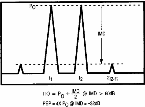
Figure 10. Intermodulation Test
