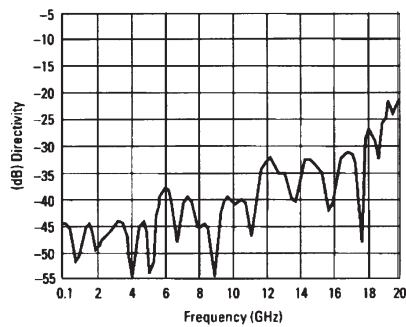
Typical directivity
