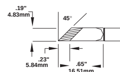
SMTC-X173 Knife (Increased Tinned Area, .23" 5.84mm)
